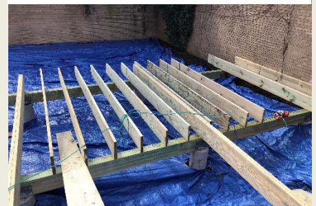
Deck Installation
